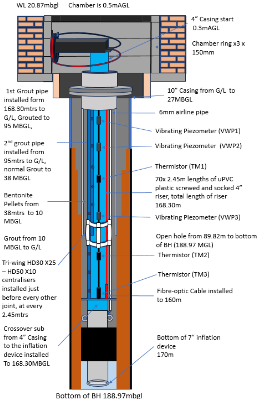
Fig. 2: Diagram of BH4a-01A Hutton
