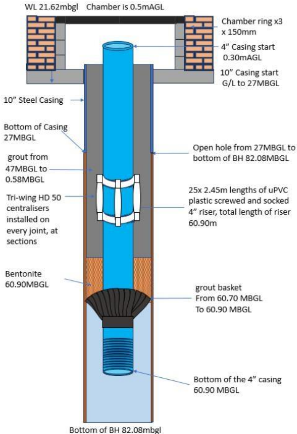
Fig.3: Diagram of BH4b-01 Stadium High Main
