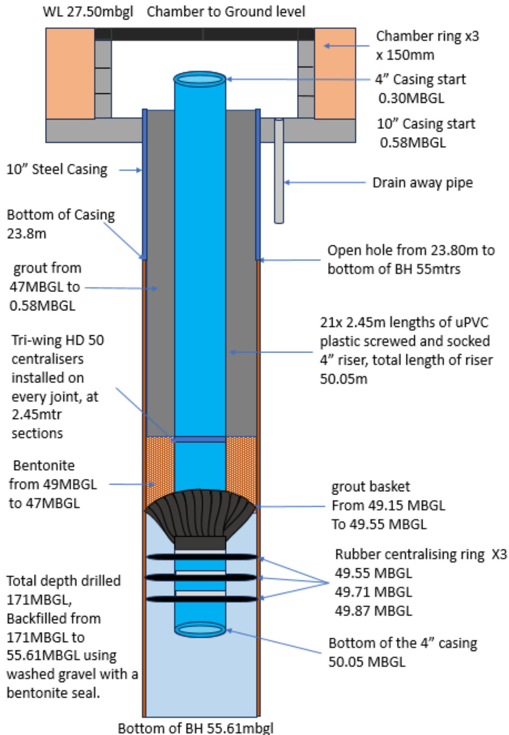
Fig.3: Diagram of BH2 and casing installation performed in June-2023
